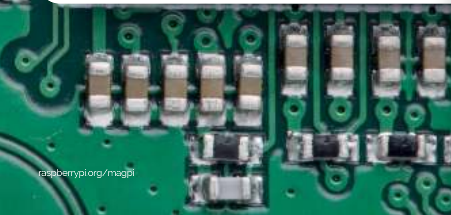
The intelligent layout enables all the circuitry to be placed on one side of the PCB, keeping the cost down
