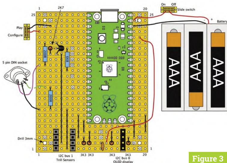
▼ Figure 3 The front of the board assembly
