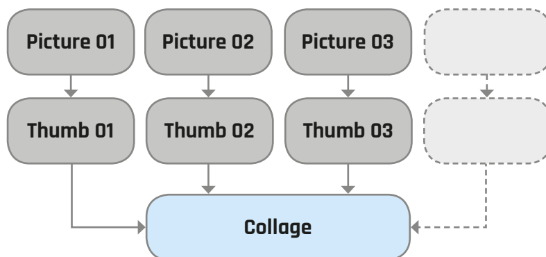
Fig 3 COLLAGE DEPENDENCY GRAPH
