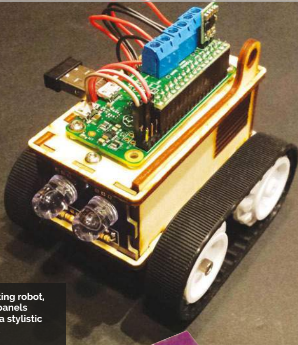
The board with the LEDs is custom-made, to cut down on wiring in the project
