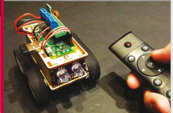
The board with the LEDs is custom-made, to cut down on wiring in the project
