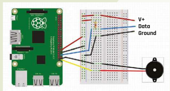
Above top Our initial circuit needs to make sure we have the thermal sensor's information
