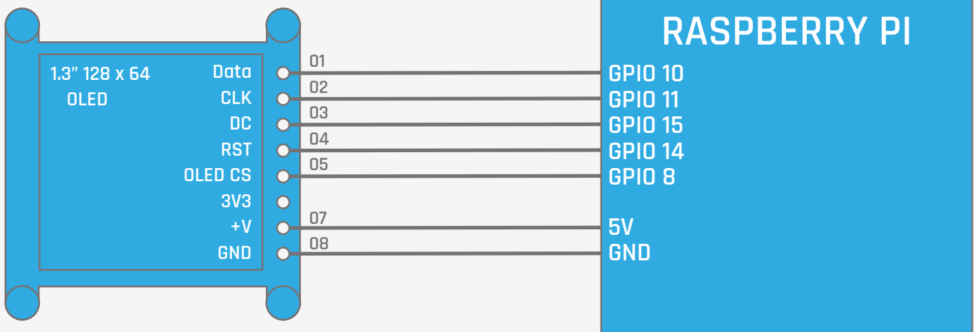
Fig 1 Connecting the OLED display to the Raspberry Pi
