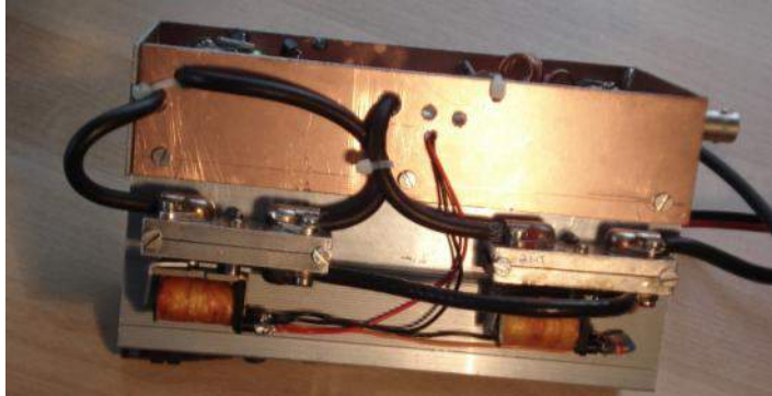
Montage coax relais
