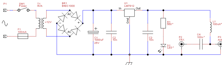
Circuit of the renewed PoRG, see text below for remarks on the components tagged with a "*" symbol.
