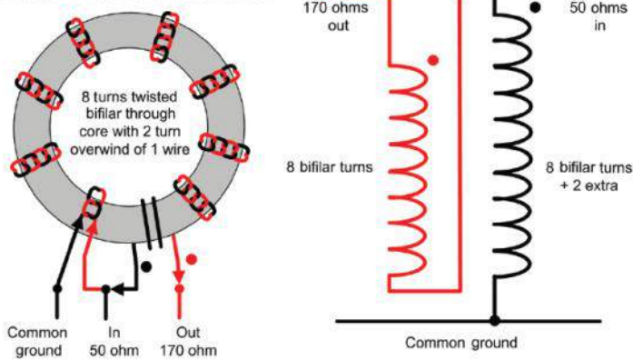
FIGURE 10: 170:50Ω unun construction.
