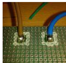
Cut away the solder pads on the circuit board wherever 230Vac is the operating voltage.
